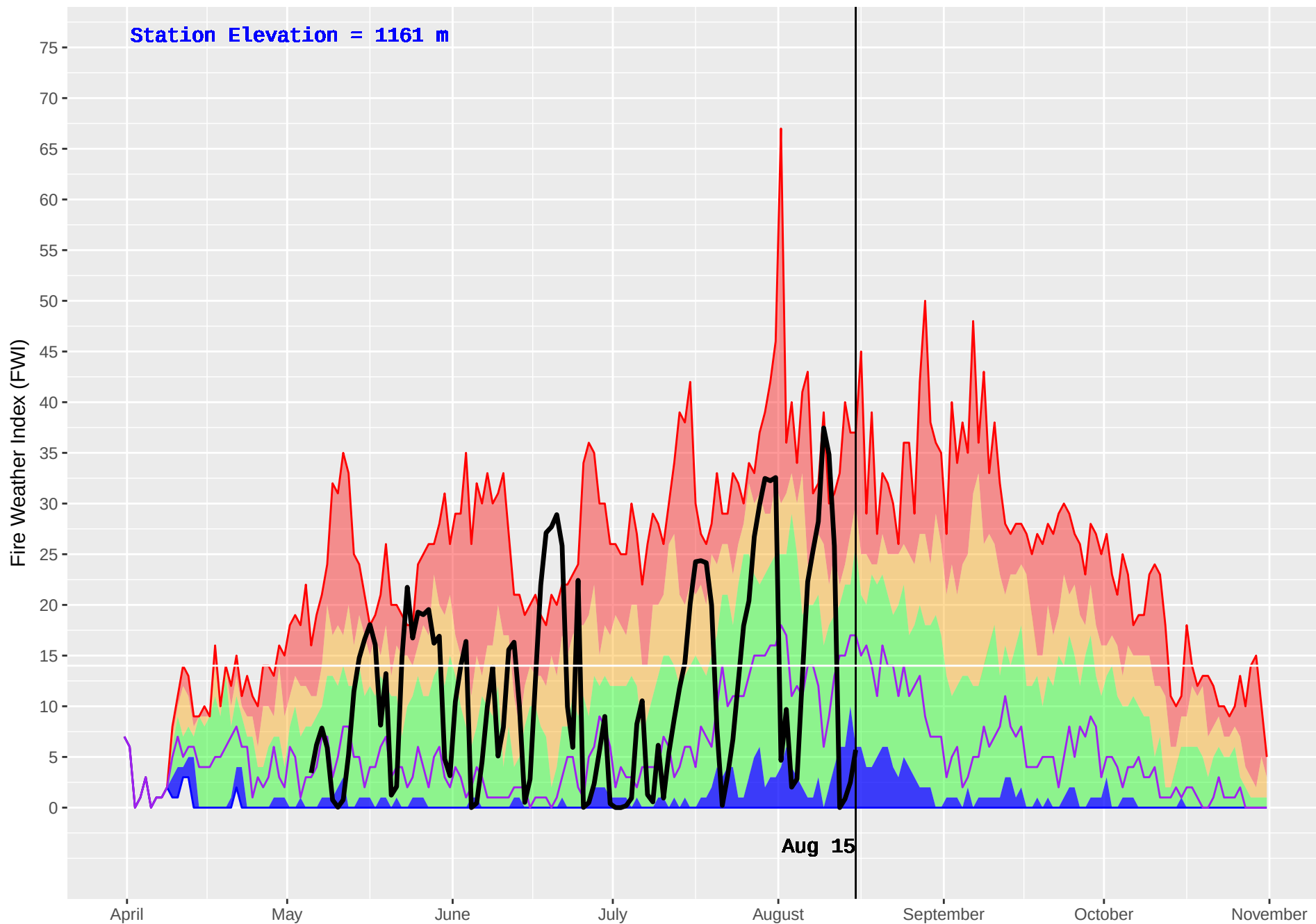
TIMOTHY (234) : Historical (1990–2016) and Current (2018) Daily Fire Weather Index (FWI)
