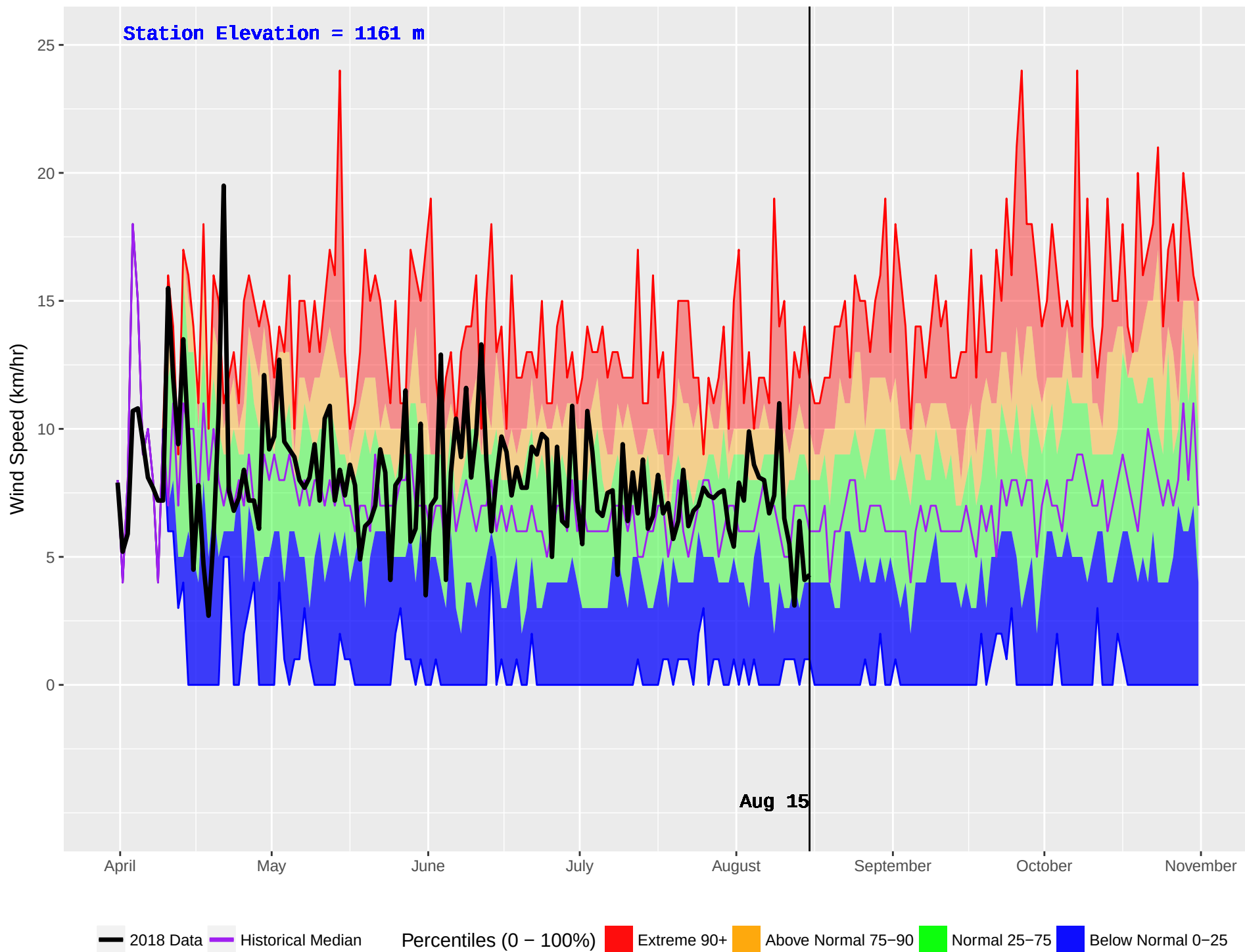
TIMOTHY (234) : Historical (1990–2016) and Current (2018) Daily Wind Speed
