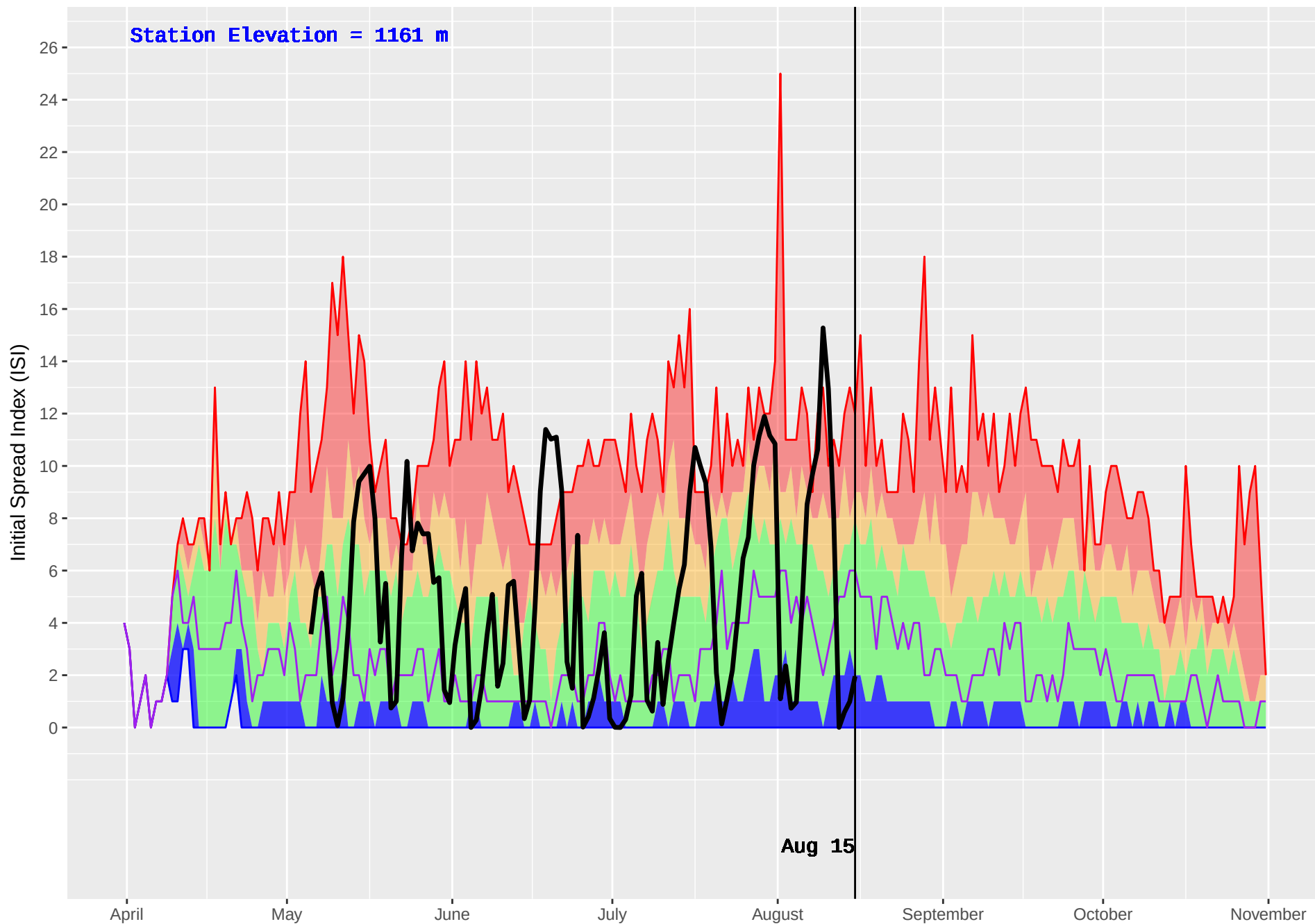
TIMOTHY (234) : Historical (1990–2016) and Current (2018) Daily Initial Spread Index (ISI)
